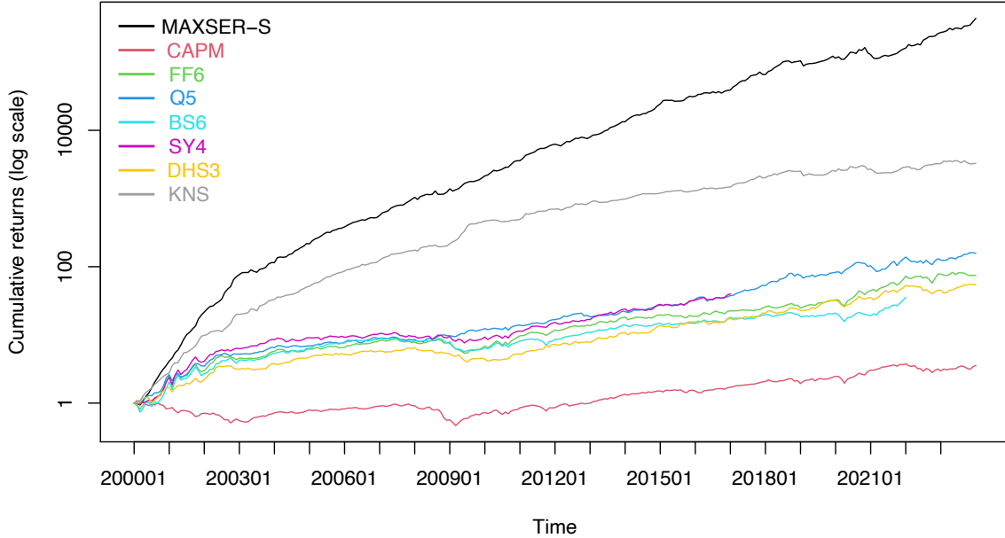
Figure 1: Cumulative dollar returns of the SDF portfolios. This figure plots the cumulative returns of various SDF portfolios from 2000 to 2023, starting with $1. We include the SDF portfolios constructed from MAXSER-S, CAPM, FF6, Q5, BS6, SY4, DHS3, and KNS. The portfolio risk is set to be the market risk.
